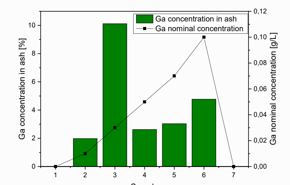
Fig. 5 Ga^{3+} Concentration nominal and measured in Ashes [2]
